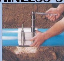
TIGHTEN NUTS EVENLY WITH WRENCH
